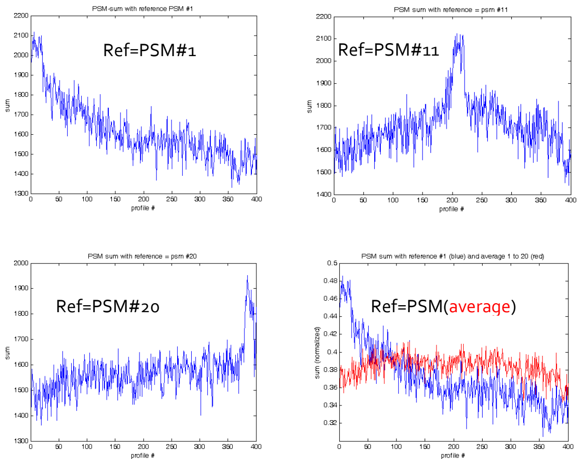
Figure 16: Three examples of the FoM (top and lower left). At the lower right the normalized FoM is shown in a comparison between PSM #1 (blue) and the average PSM (red).
