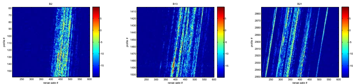
Figure 17: measured HRR profiles (dB) for three distance intervals B2, B13, B21 (100 profiles corresponding to 25m) lying about 350m apart
